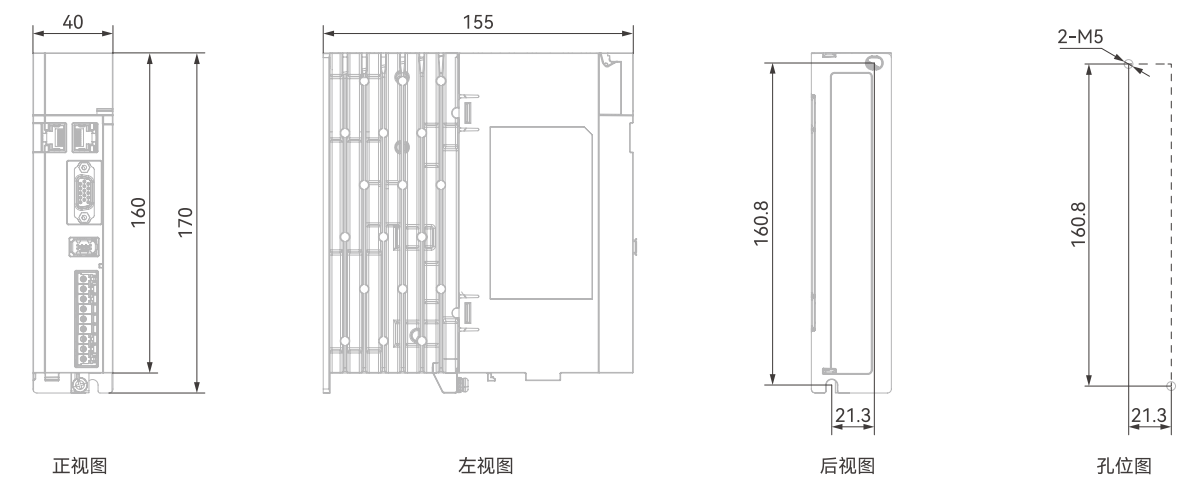
Size B整机外形尺寸 (mm)
