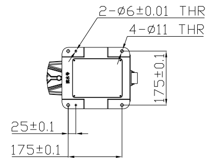
底部安装孔 Bottom mounting hole
