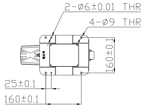
底部安装孔 Bottom mounting hole
