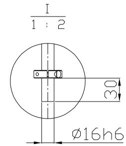
外设夹具安装轴径 Peripheral fixture mounting axle diameter
