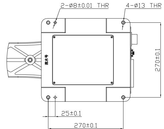
底部安装孔 Bottom mounting hole
