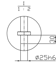
外设夹具安装轴径 Peripheral fixture mounting axle diameter
