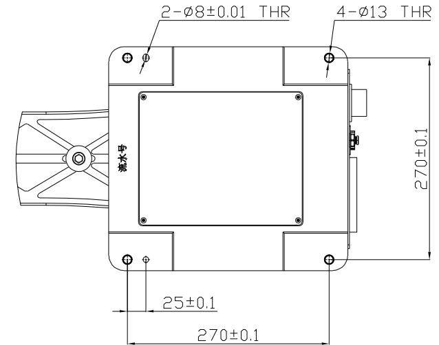
底部安装孔 Bottom mounting hole
