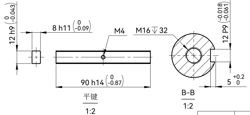
电机动力端 Motor Power Connection
