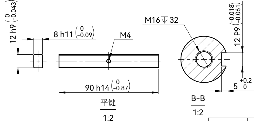
编码器端 Encoder Connection
