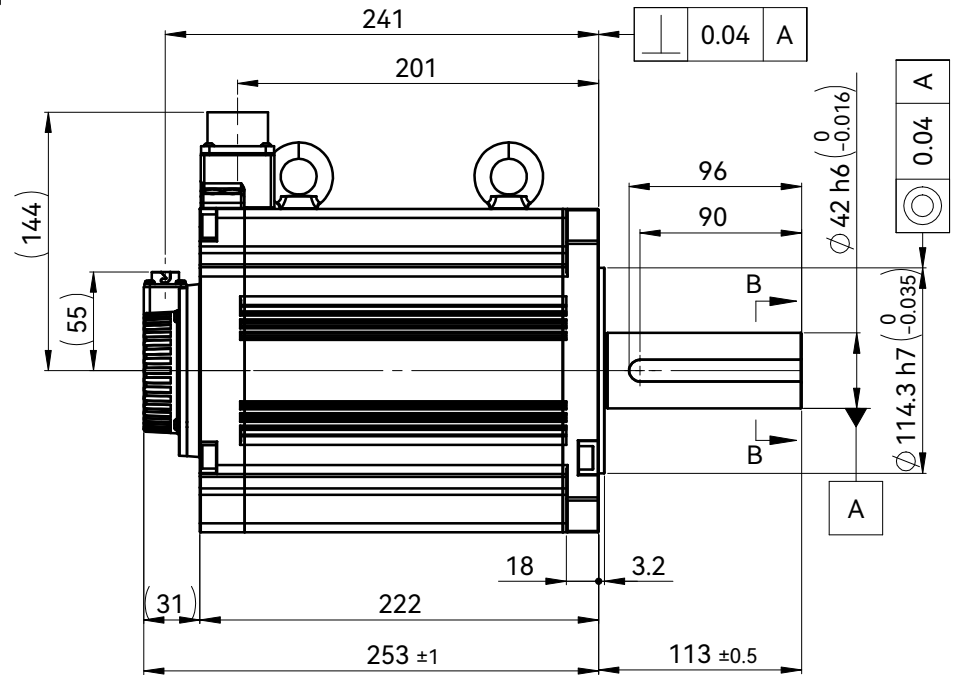
电机动力端 Motor Power Connection
