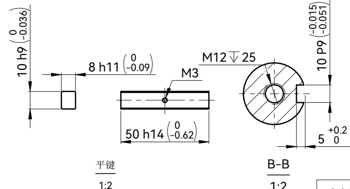
编码器端 Encoder Connection
