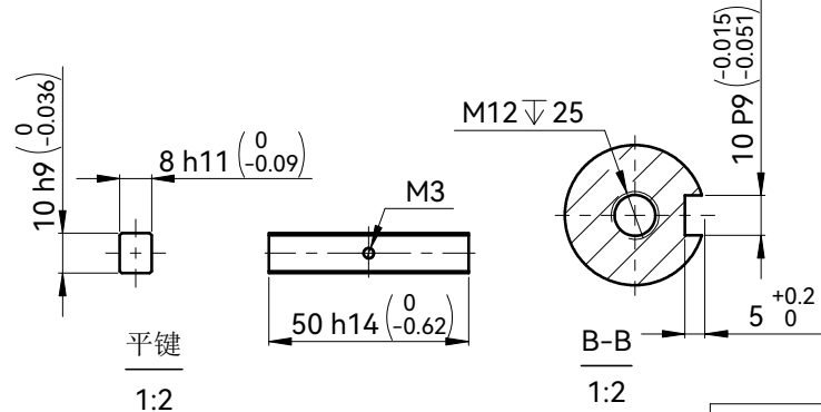
编码器端 Encoder Connection
