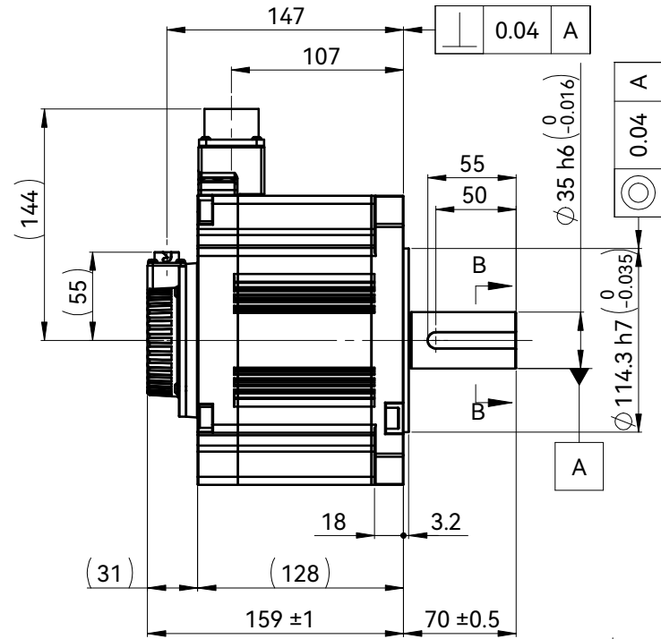
电机动力端 Motor Power Connection
