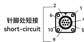
信号线插头: Encoder connector:
