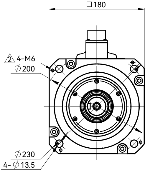
电机动力端Motor Power Connection
