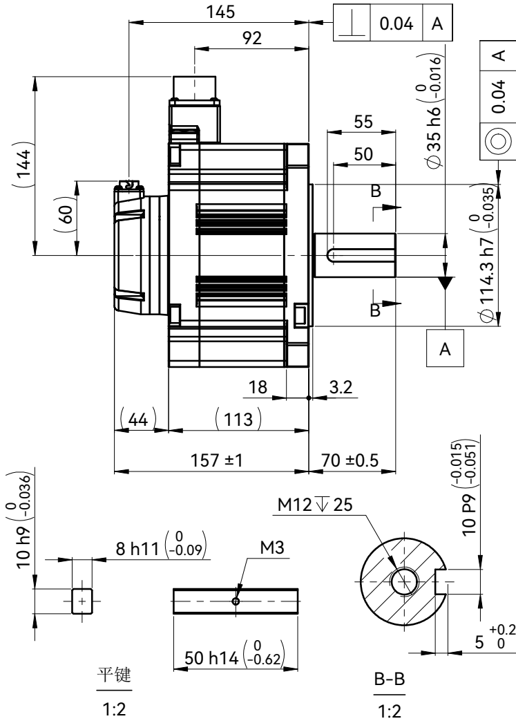
电机动力端Motor Power Connection
