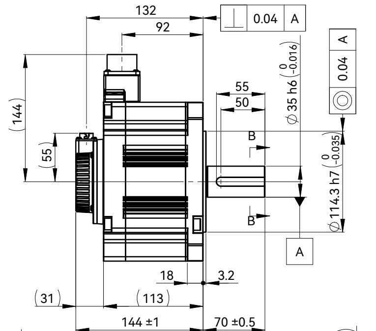
电机动力端 Motor Power Connection
