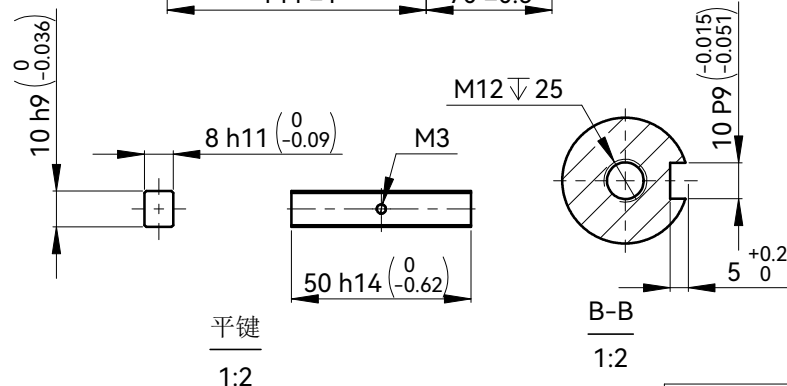
电机动力端 Motor Power Connection
