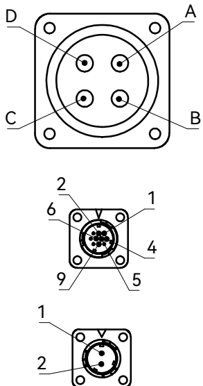
编码器端 Encoder Connection
