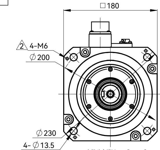
电机动力端 Motor Power Connection
