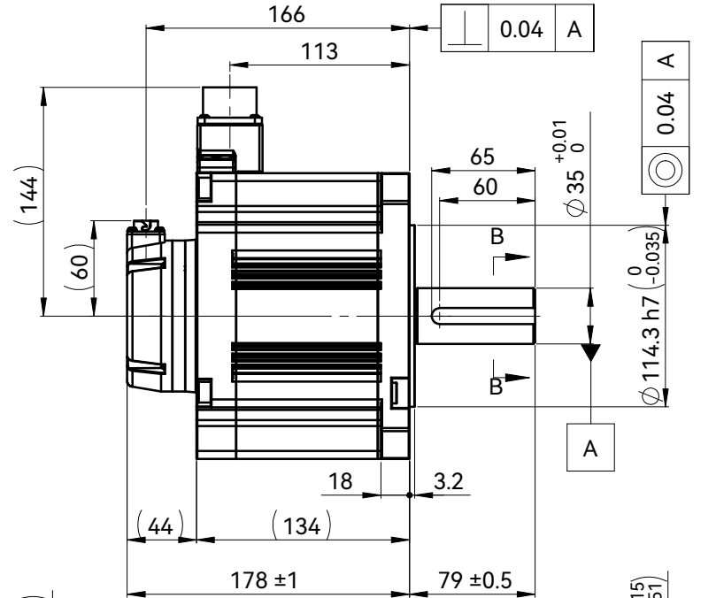
电机动力端 Motor Power Connection
