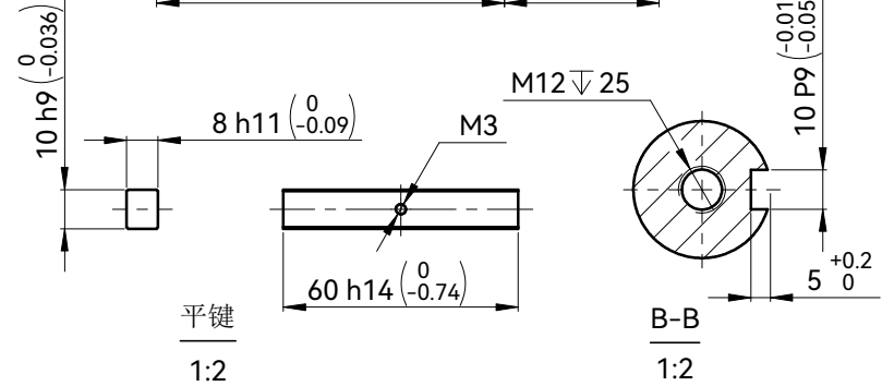
电机动力端 Motor Power Connection
