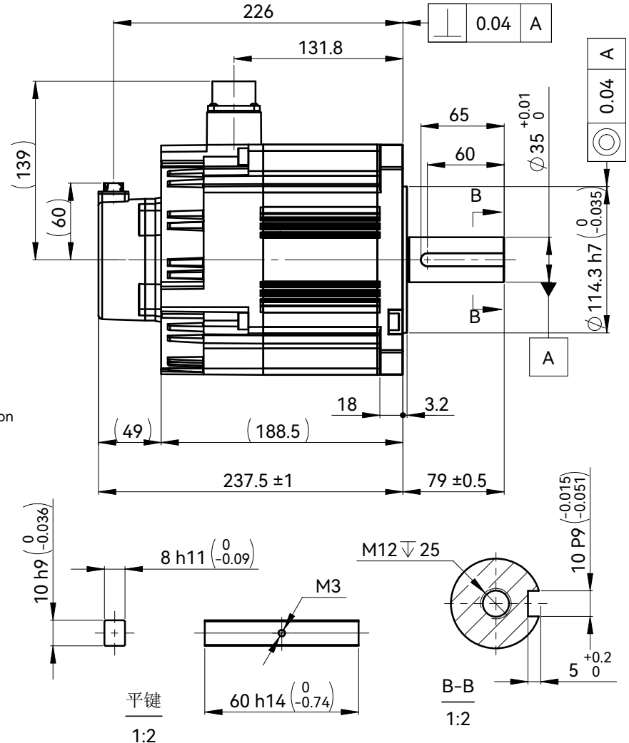
编码器端 Encoder Connection
