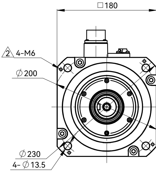
电机动力端 Motor Power Connection
