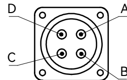
编码器端 Encoder Connection
