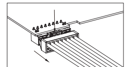
按压锁扣并拔出端子 Press the latch and detach the terminal block
