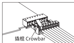
安装撬棍 Install the crowbar
